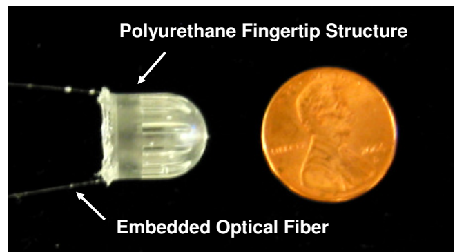
Fig. 11. Miniaturized polyurethane finger prototype fabricated as a hollow shell composed of several curved ribs that are connected at the base by a circular ring and meet at the apex. Optical fibers with FBG sensors are embedded in the ribs.
