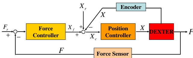
Fig. 8. Position Based Smart Force Control System
