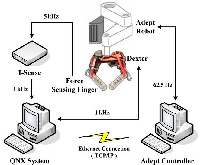
Fig. 6. Overall Hardware System Architecture
