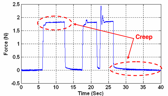
Fig. 4. Testing the effect of applying a steady load for several seconds and suddenly removing it from the polymer fingertip. Figure 5 shows detailed views of typical loading and unloading periods.
