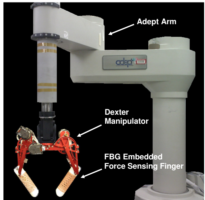
Fig. 1. FBG embedded force sensing finger prototypes integrated with Dexter manipulator and Adept robot arm
