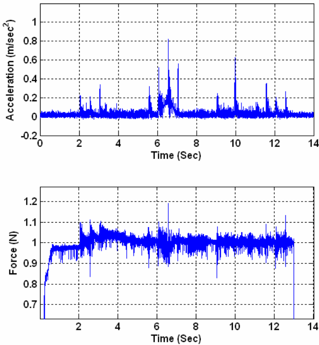
Fig. 10. Force control data during a manipulation task (bottom). Magnitude of combined (x, y, and z) acceleration of the robot is plotted along with the grasp force measured by a finger with FBG sensors (Top).
