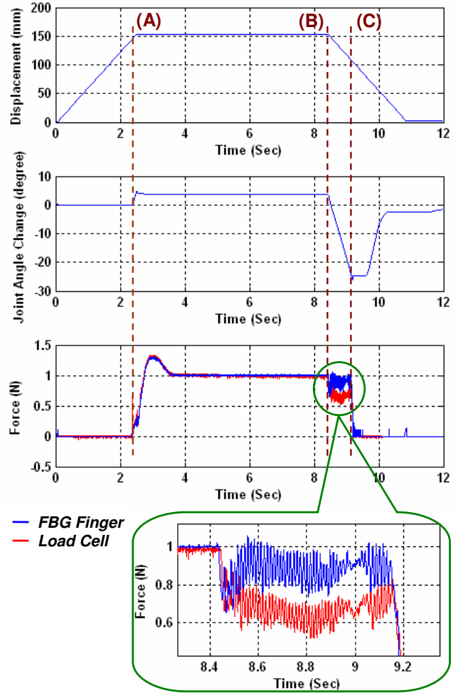
Fig. 9. (Top) Adept robot motion, (Middle) Joint angle change of Dexter manipulator, (Bottom) Force data from load cell and FBG embedded robot finger prototype; (A) Robot makes a contact, (B) Robot starts retreat, (C) Robot loses the contact.
