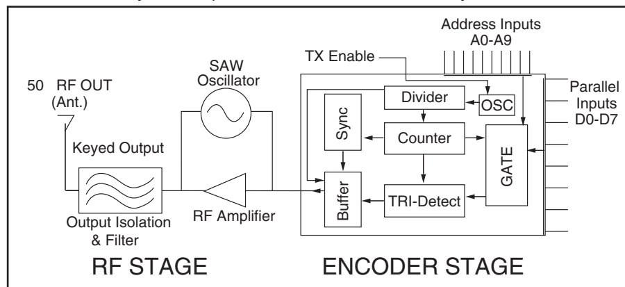
Figure 7: KH Series Transmitter Block Diagram
