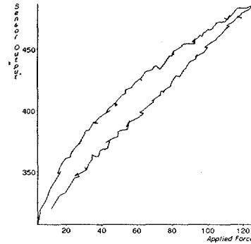
Figure 4: Tactile sensor output versus applied force.
