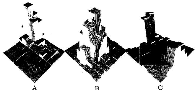
Figure 5: Force response to blunt tipped probes, from left to right: small probe, large probe, two probes at each end of the pad.
