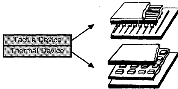
Figure 1: Contact Sensor Design. Left: cross section of sensor. Right: exploded views of the tactile (upper) and thermal (lower) devices
