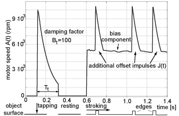
Figure 4. Motor rotation speed while tapping and stroking over an object surface.
