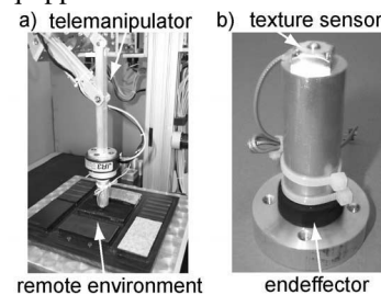
Figure 12. Texture sensing in RE.
