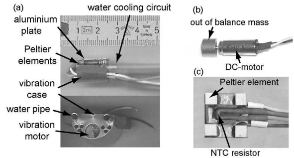
Figure 2. Tactile fingertip feedback module.
