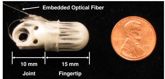
Fig. 11. Miniaturized polyurethane finger prototype fabricated as a hollow shell composed of several curved ribs that are connected at the base by a circular ring and meet at the apex. One optical fiber with four FBG sensors is embedded in the ribs.
