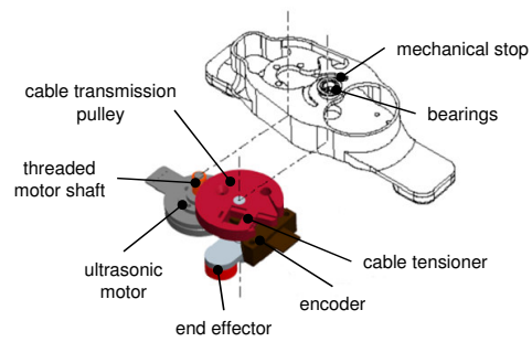
Figure 2: Skin Stretch Device
